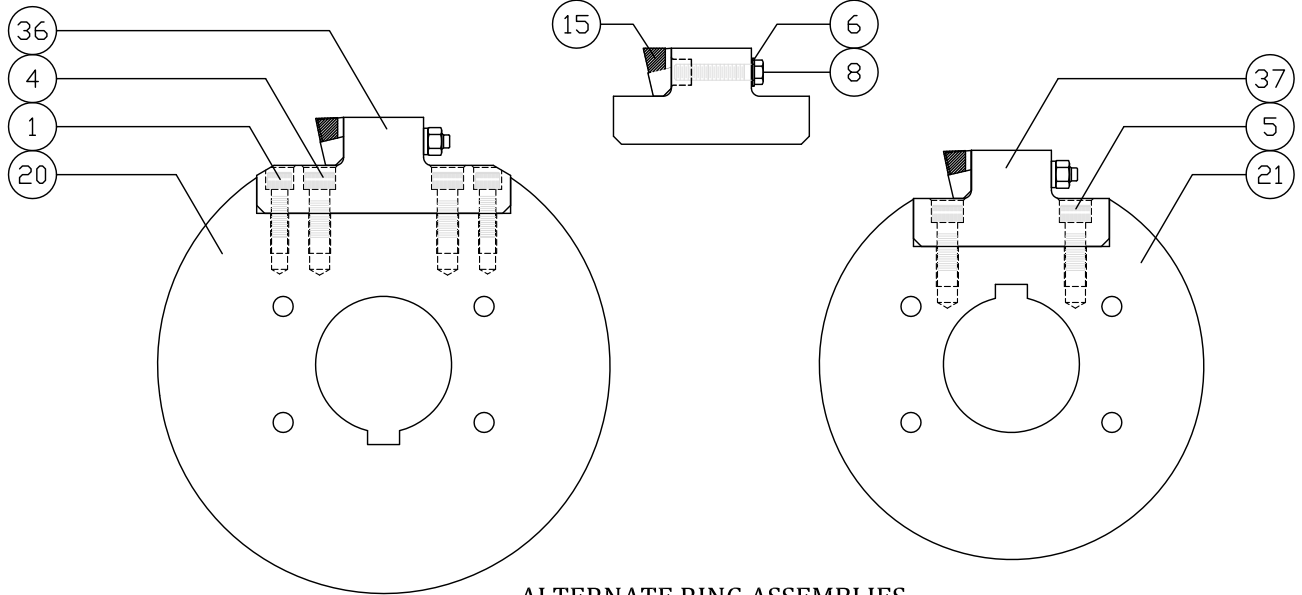
ALTERNATE RING ASSEMBLIES SHOWING LUG INSERTS IN LIEU OF FIXED LUG TYPE RINGS.
