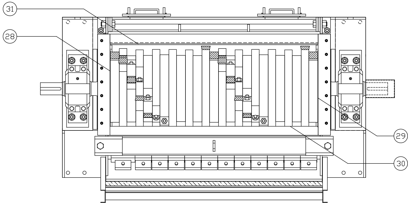
ALTERNATE DOOR 24" FEED OPENING
