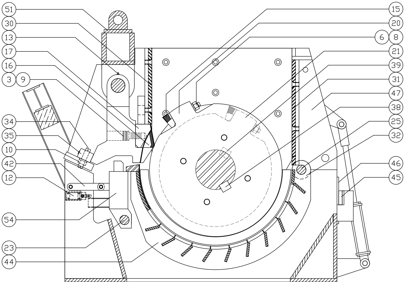
ALTERNATE RING ASSEMBLIES SHOWING LUG INSERTS IN LIEU OF FIXED LUG TYPE RINGS.
