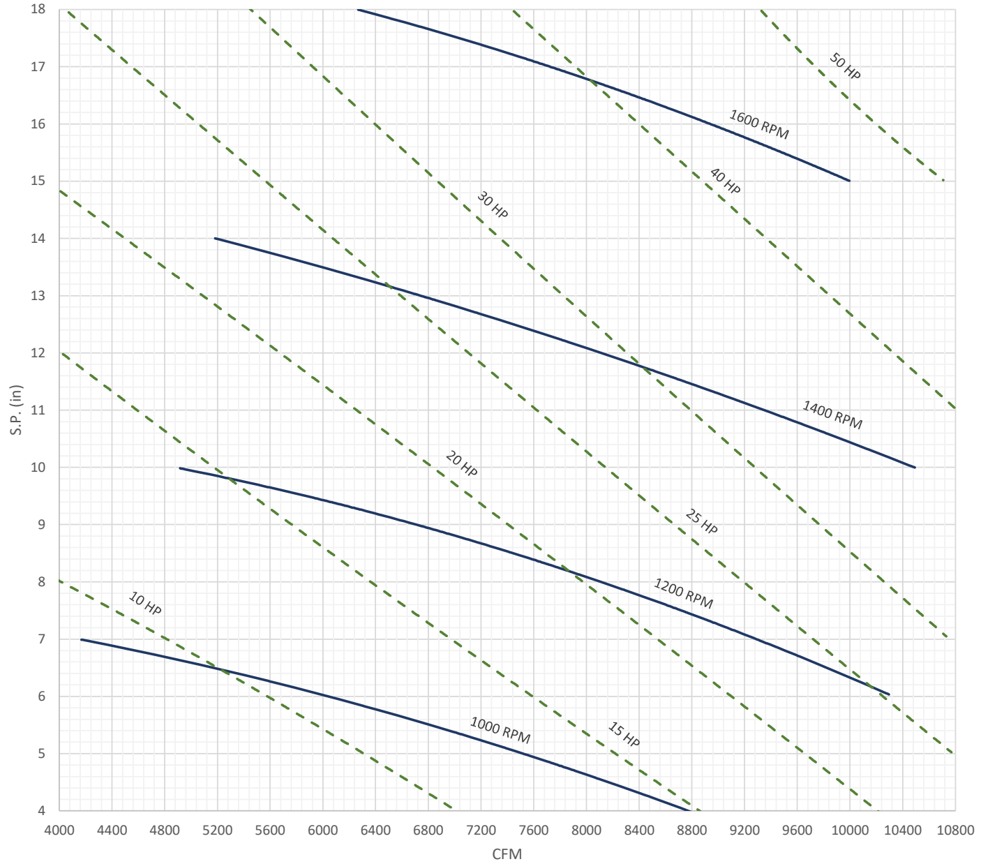
No. 40 Fan Performance Curves
