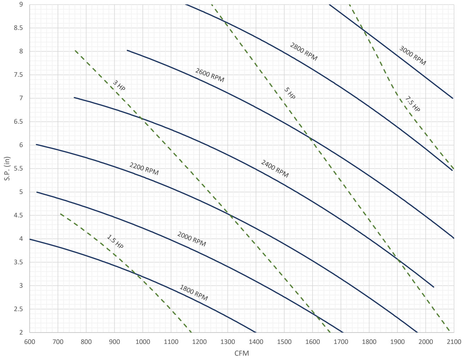
No. 18 Fan Performance Curves
